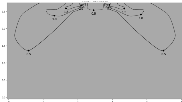
Figure 9.3: MIH22Q4CHN18 cooling at 300s
