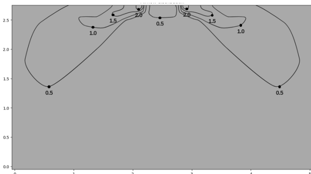
Figure 9.5: MIH28Q4CHN18 cooling at 300s
