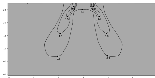
Figure 9.6: MIH28Q4CHN18 heating at 300s
