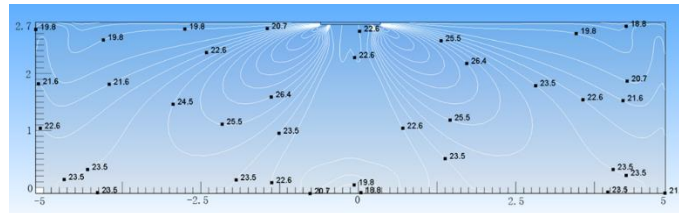
Figure 9.40: MI2-140Q4DHN1 heating at 120S
