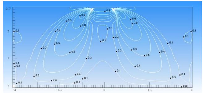
Figure 9.2: MI2-28Q4DHN1 heating at 120S
