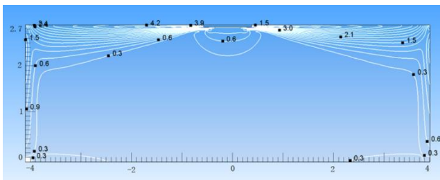
Figure 9.9: MI2-71Q4DHN1 cooling at 120S
