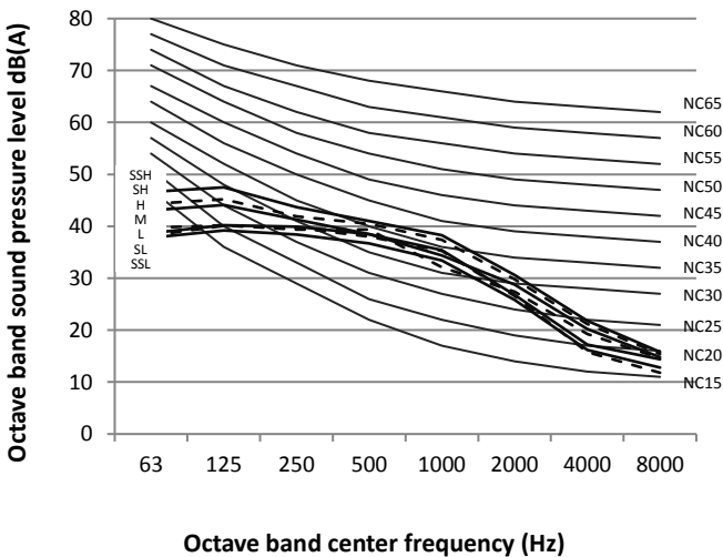
Figure 8.8: MI2-140Q4DHN1 octave band levels
