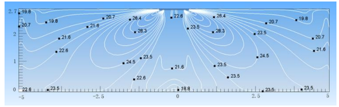
Figure 9.38: MI2-112Q4DHN1 heating at 120S
