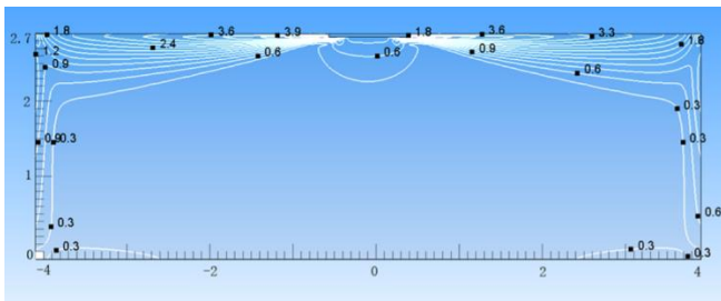
Figure 9.7: MI2-56Q4DHN1 cooling at 120S
