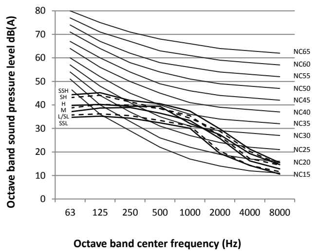
Figure 8.7: MI2-100(112)Q4DHN1 octave band levels
