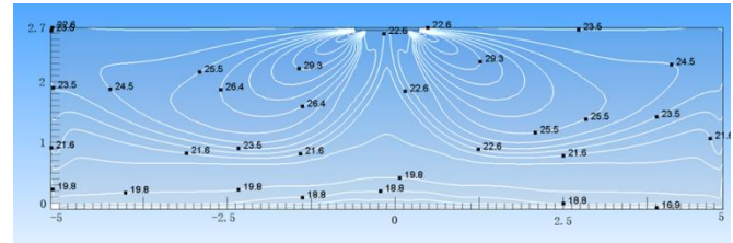
Figure 9.34: MI2-90Q4DHN1 heating at 120S
