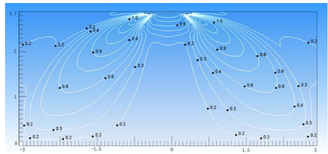
Figure 9.6: MI2-45Q4DHN1 heating at 120S
